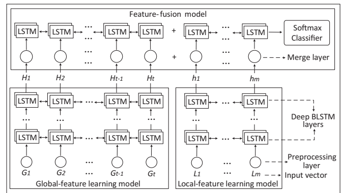
Fig. 4. The \mu VulDeePecker neural network architecture.
