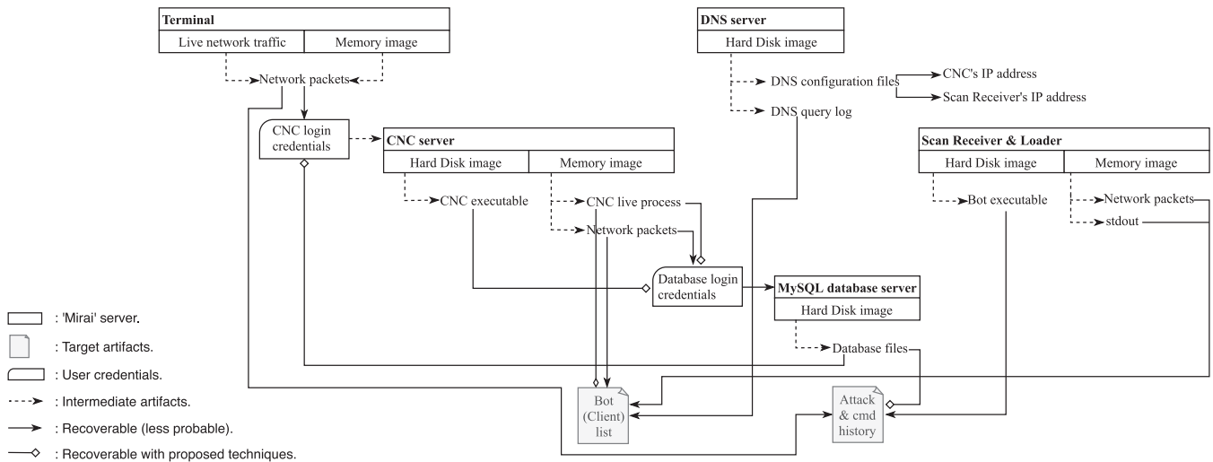
Fig. 14. The road map for Mirai botnet server forensics.
